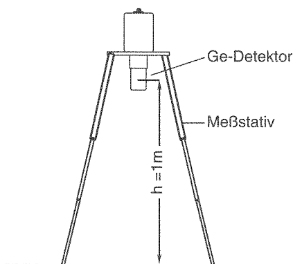
Abb. 1: In situ Gamma-Spektrometer in Meßposition (8)
