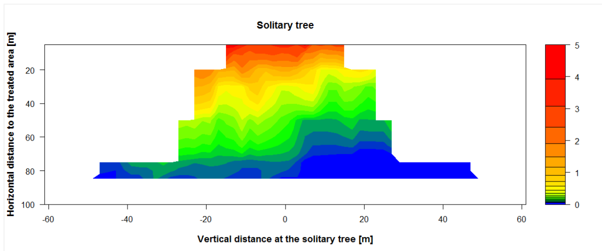
Figure 8: Surface distribution of the ground sediment in percent of the application rate at the cannon sprayer application at a solitary tree based on maximum values.
